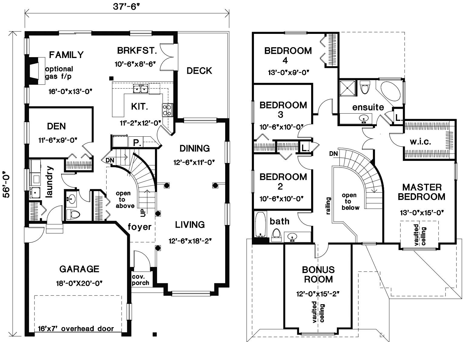
The HAMPTON 2,610 sq. ft. BONUS room 205 sq. ft.
