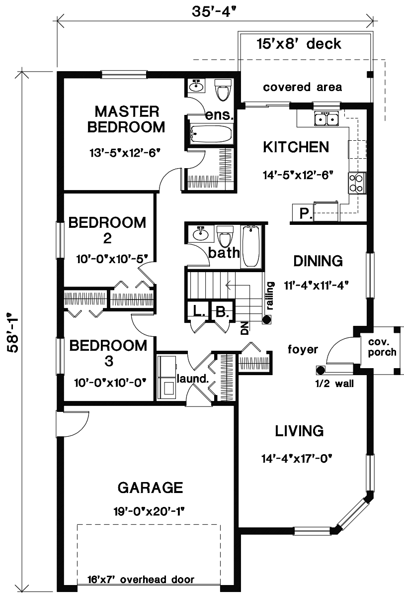
The ERINDALE 1,475 sq. ft.
