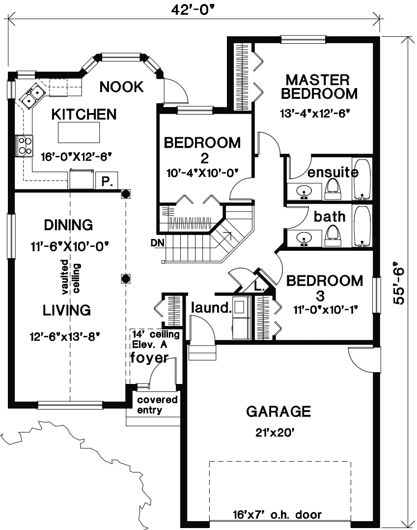
Plan A
